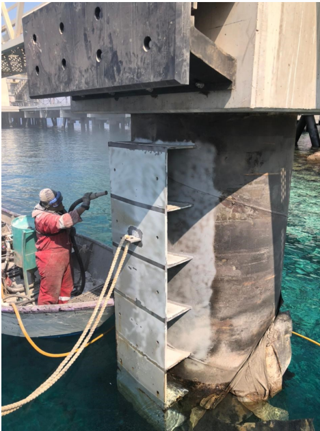
Marine Fender Back Structure
